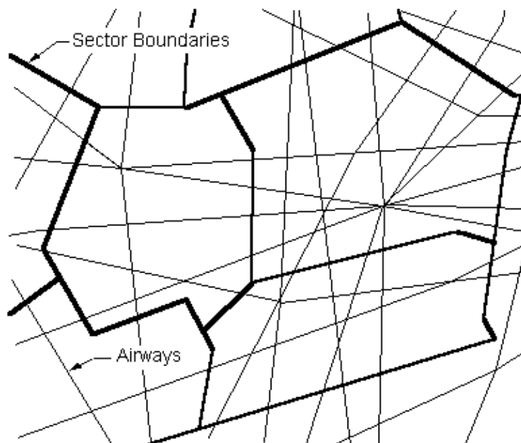
Figure 8. Indianapolis ARTCC High Altitude Sectors and Airways
