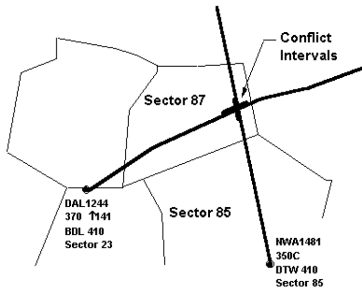
Figure 9. An Alert Notified to Sector 87 14 Minutes Before the Start of Conflict
